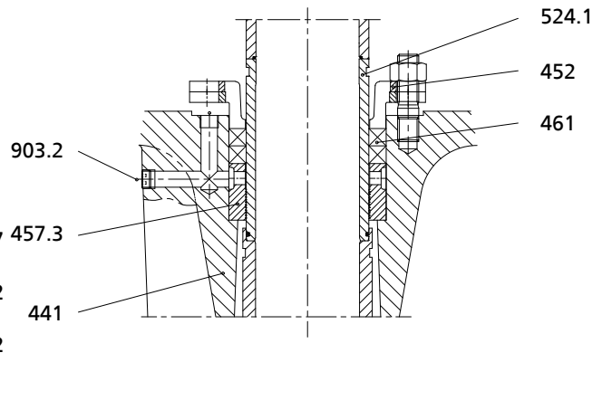
Detailed view: gland packing, pump discharge pressure \geq 7 bar [99.5 psi]
